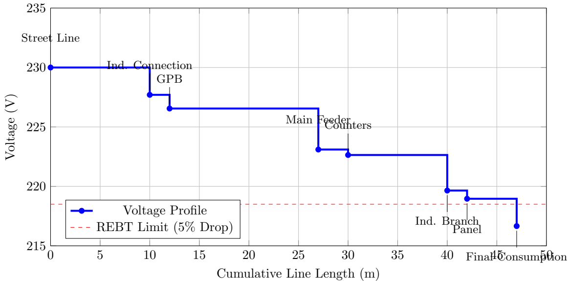
Voltage Profile Across Multi-Segment Installation
